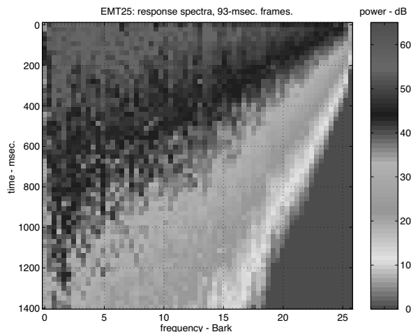
Figure 5: CCRMA Lobby Impulse Response STFT.
