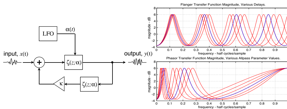
Figure 7: Flanger/Phasor Architecture, Example Transfer Functions.
