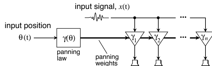
Figure 9: Multichannel Panning.
