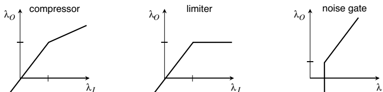
Figure 3: Compressor, Limiter and Noise Gate Input Level-Output Level Relationships.
